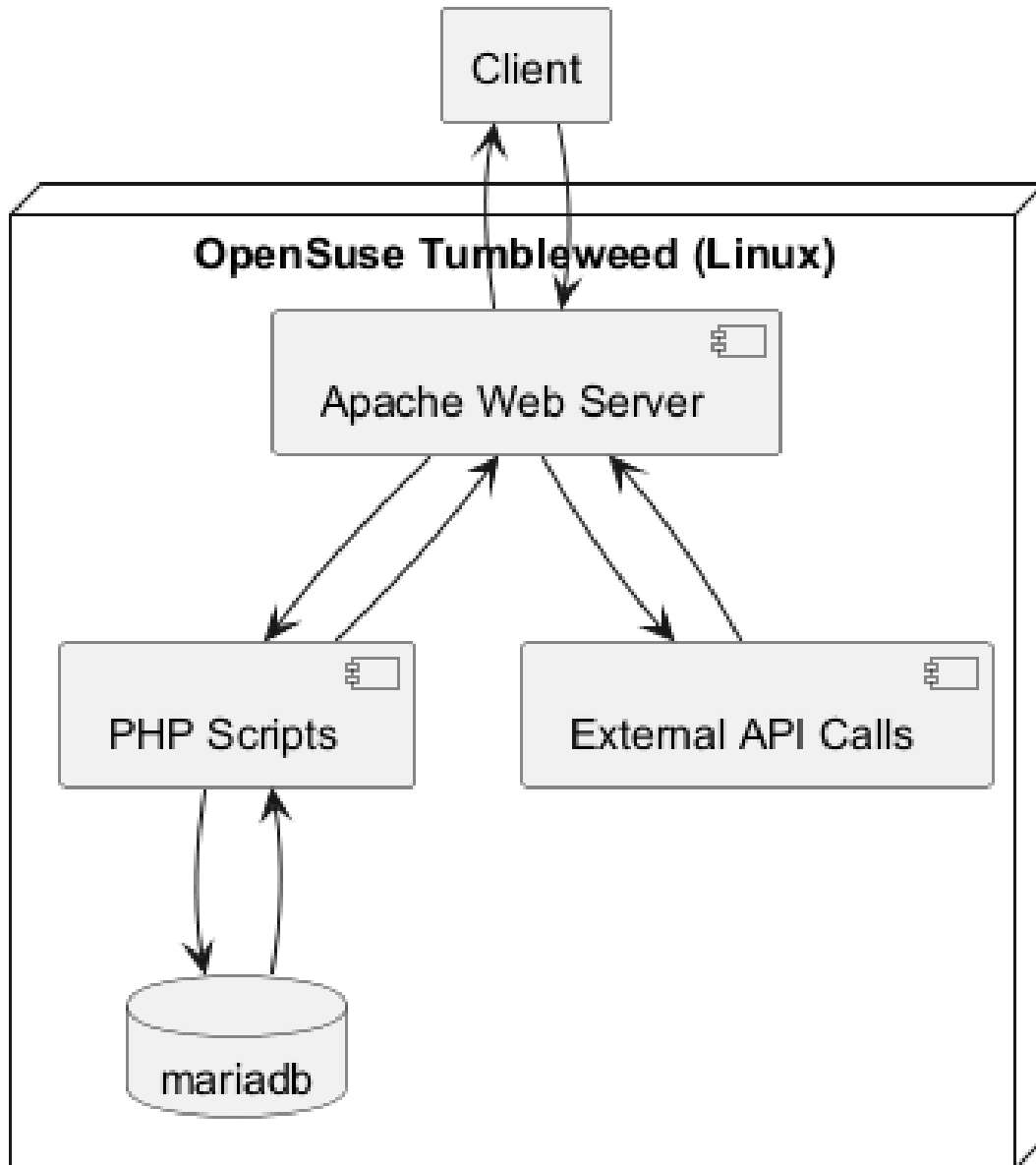
Figure 3: System Architecture Diagram
